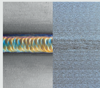
Saldature TIG decapate e spazzolate TIG welding pickled and passivated Nettoyage mecanique de soudures TIG
